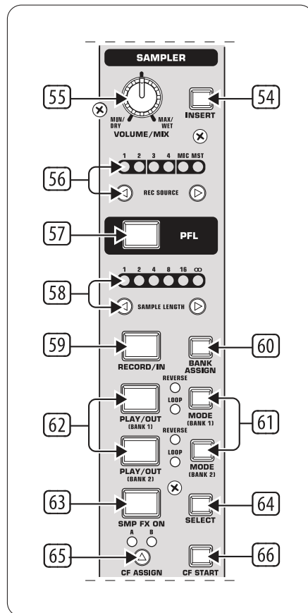
Fig. 10: Sampler section
